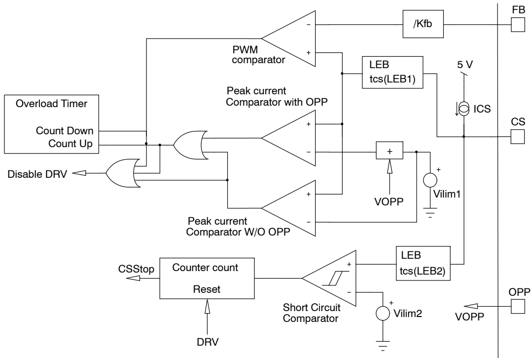
Figure 57. Overload Circuitry
