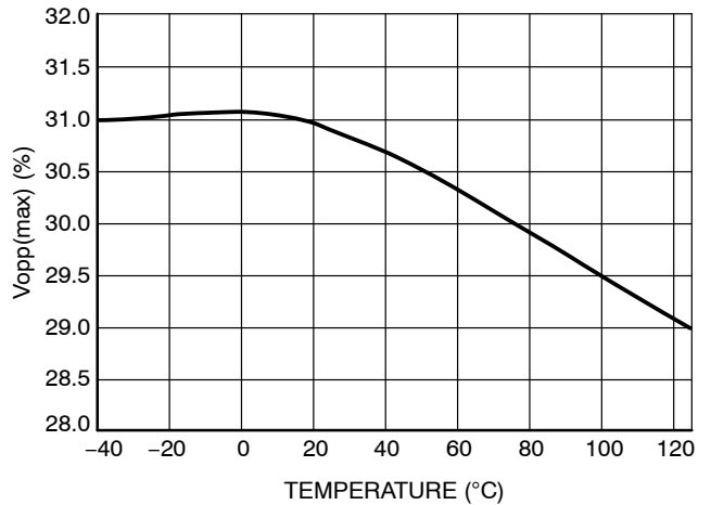
Figure 39. V_{OPP(MAX)} vs. Junction Temperature
